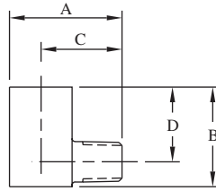
Street Elbow
